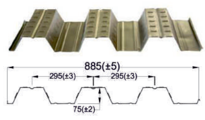
LCP FORMDEK® 75
