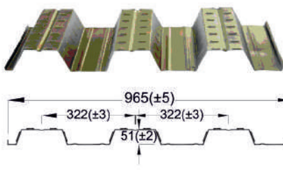
LCP FORMDEK® 51
