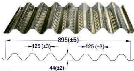
LCP FORMDEK® 44
